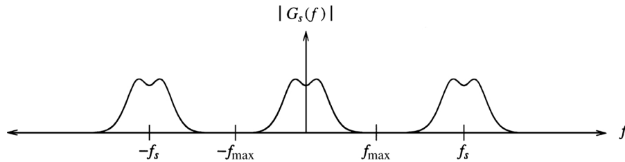
FIGURE 39.3 Spectrum G_s(f) .
