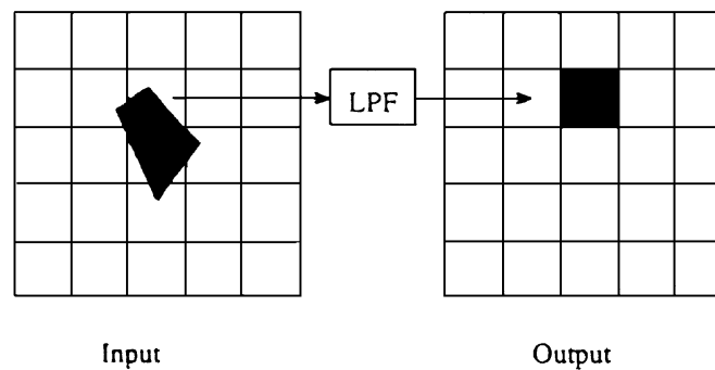
FIGURE 39.20 Area sampling.
