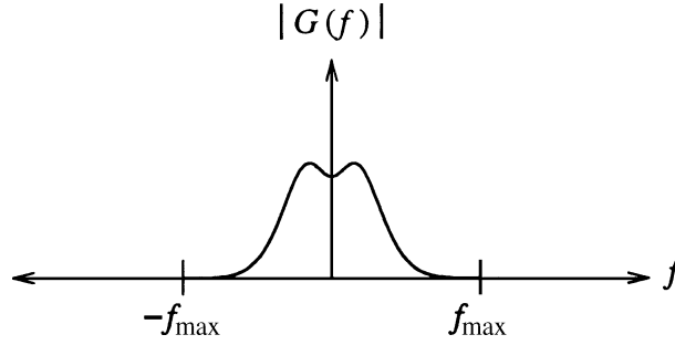
FIGURE 39.2 Spectrum G(f) .
