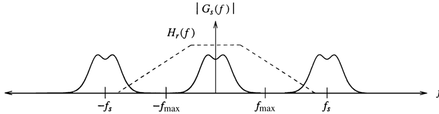
FIGURE 39.7 Nonideal reconstruction.
