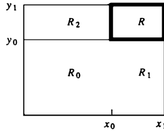
FIGURE 39.24 Summed-area table calculation.
