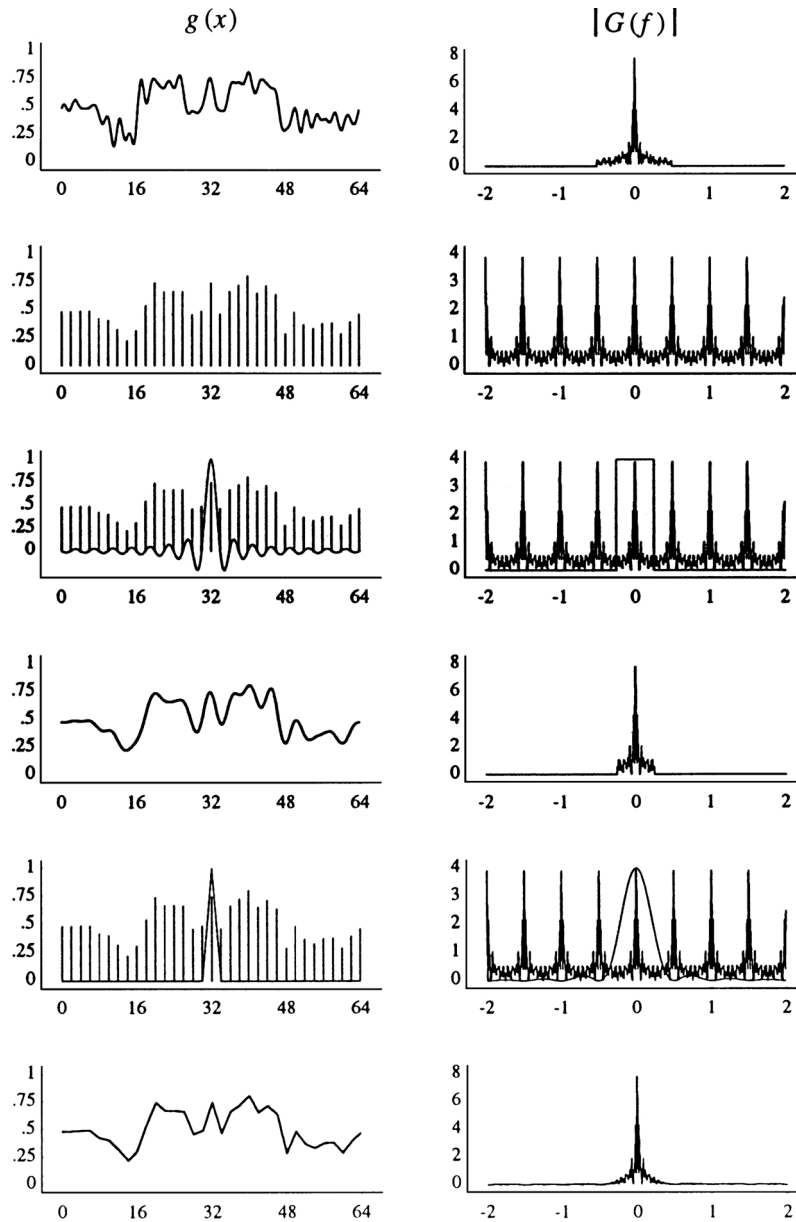
FIGURE 39.26 Sampling and reconstruction (with an inadequate sampling rate).
