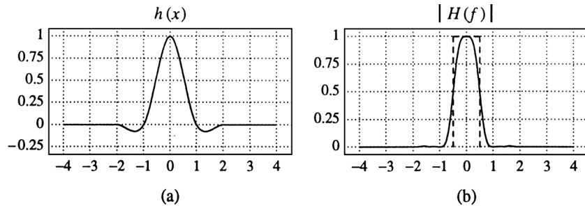
FIGURE 39.11 Cubic convolution: (a) kernel ( a = -0.5 ), (b) Fourier transform.
