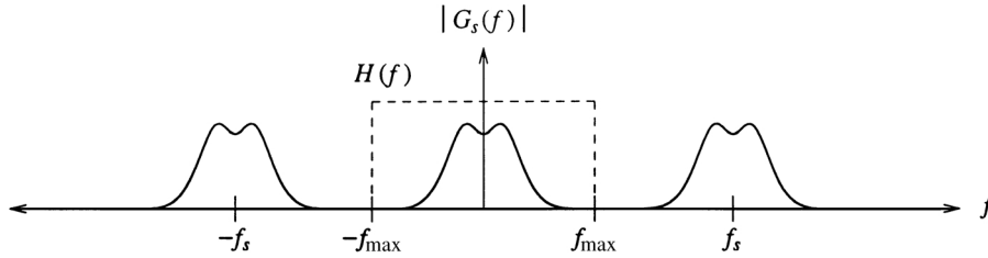
FIGURE 39.4 Ideal low-pass filter H(f) .
