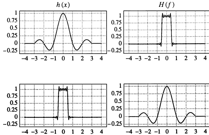
FIGURE 39.6 Truncation in one domain causes ringing in the other domain.
